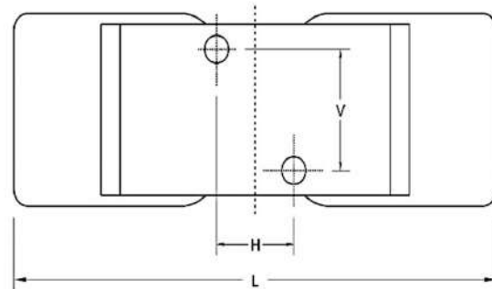
Mounting Dimensions of DTNL Series
